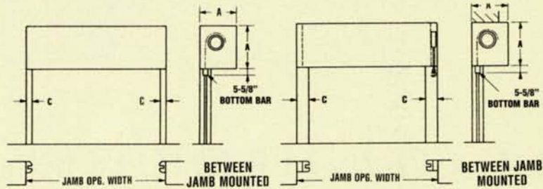
Type LDW-2 — PUSH-UP Between Jamb Mounted
