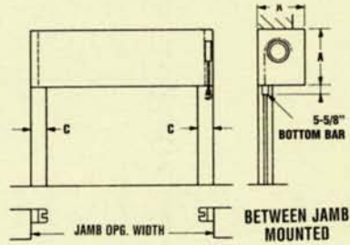
Type LDW-4 — CRANK or MOTOR Between Jamb Mounted
