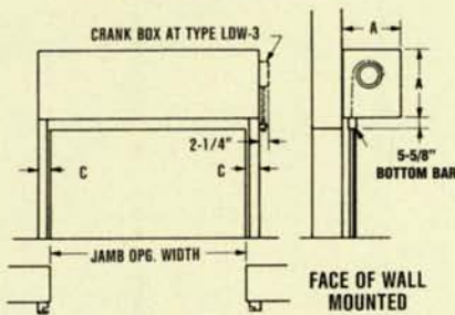
Type LDW-1 — PUSH-UP Type LDW-3 — CRANK or MOTOR Face of Wall Mounted
